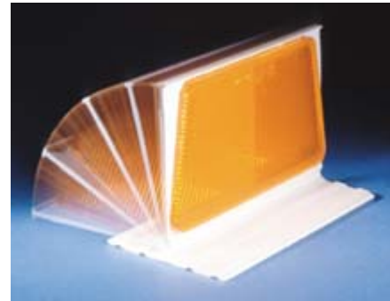
The BAM Highway Barrier Delineator has a unique hinge design that allows for full 90 degrees of flex when impacted!
