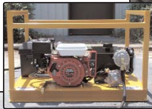
Power Pack
